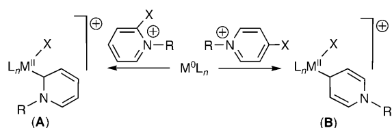
Scheme 1. Syntheses of complexes containing “normal” ( A ) and “remote” ( B ) pyridylidene ligands derived from halopyridinium cations.
